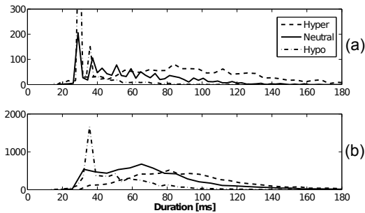
Figure 7: Phone durations histograms. (a) semi-vowels. (b) trill consonants.
